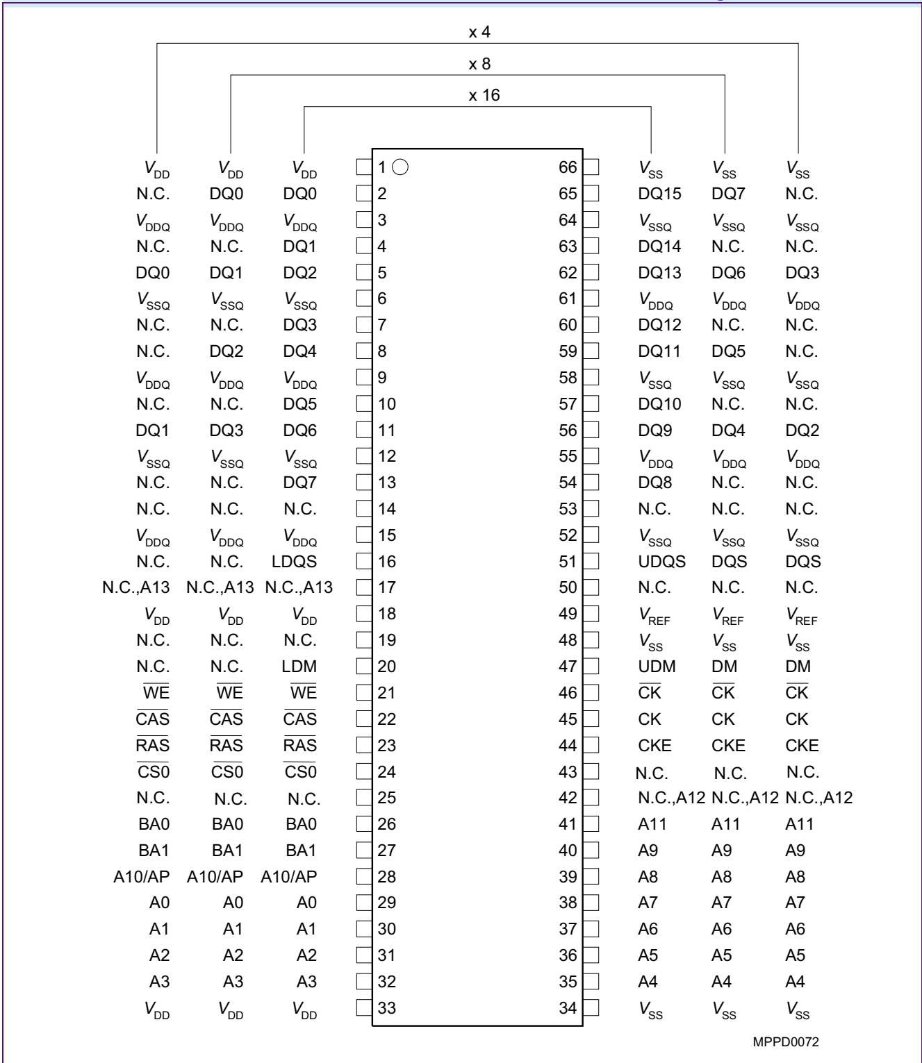
FIGURE 2 Pin Configuration P-TSOPII-66-1
