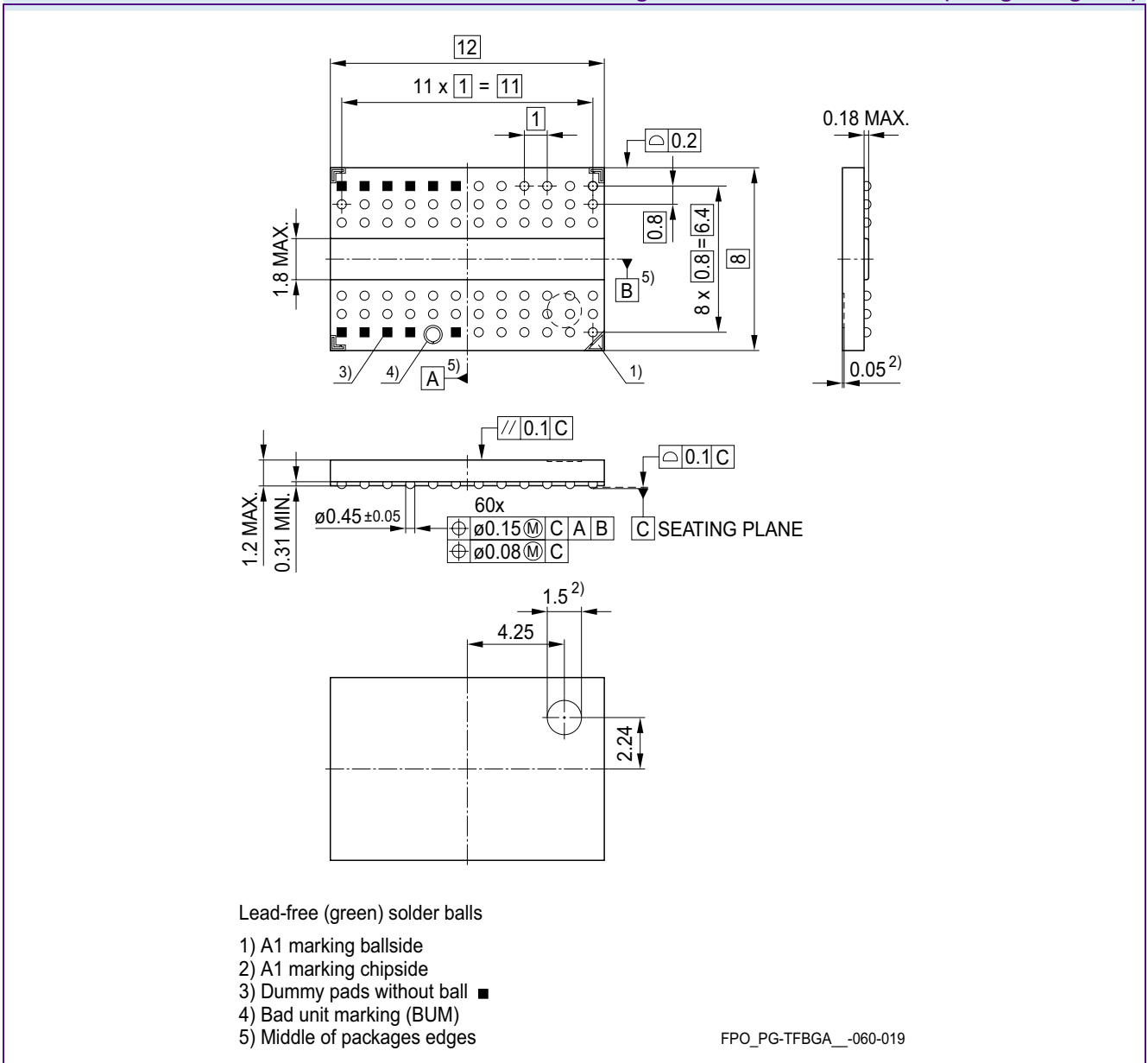
FIGURE 5 Package Outline of PG-TFBGA-60 (non-green/green)
