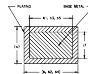
SECTION C-C, D-D, E-E
