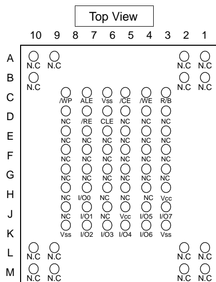
K9F1G08U0D-BCB0/BIB0
