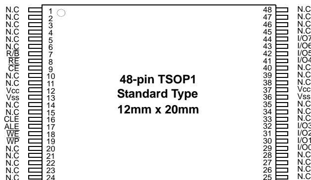
K9F1G08U0D-SCB0/SIB0
