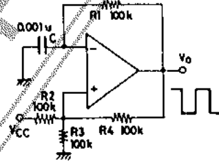
Square wave oscillator
