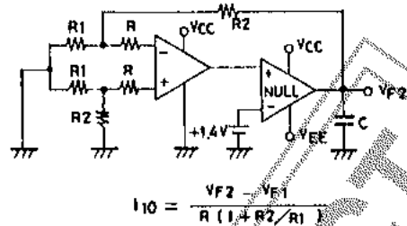
2 Input offset current I_{IO}
