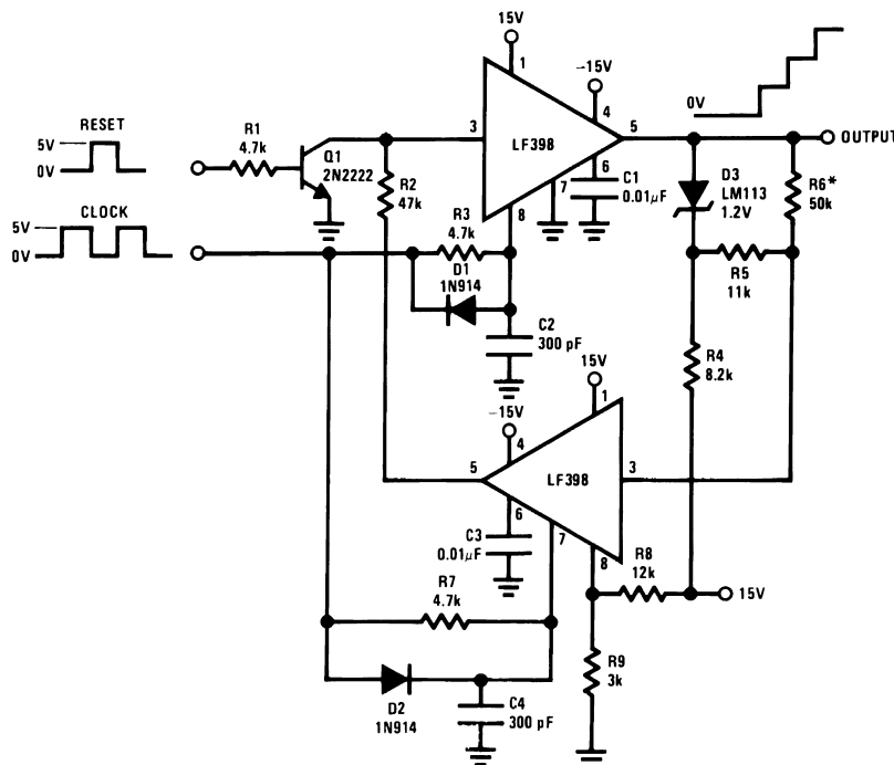
Figure 38. Staircase Generator
