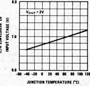
Minimum Input Voltage vs Junction Temperature
