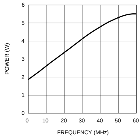
Figure 5. Power Dissipation vs Frequency
