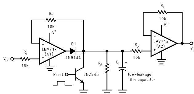
FIGURE 7. Peak Detector
