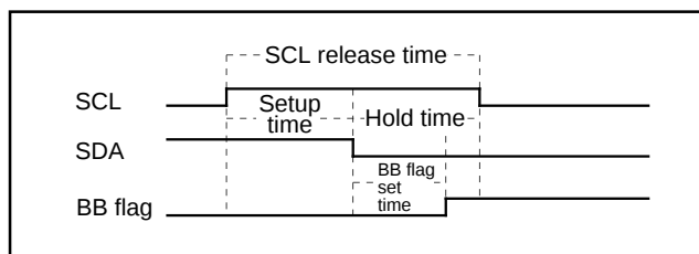
Fig. 35 START condition detecting timing diagram
