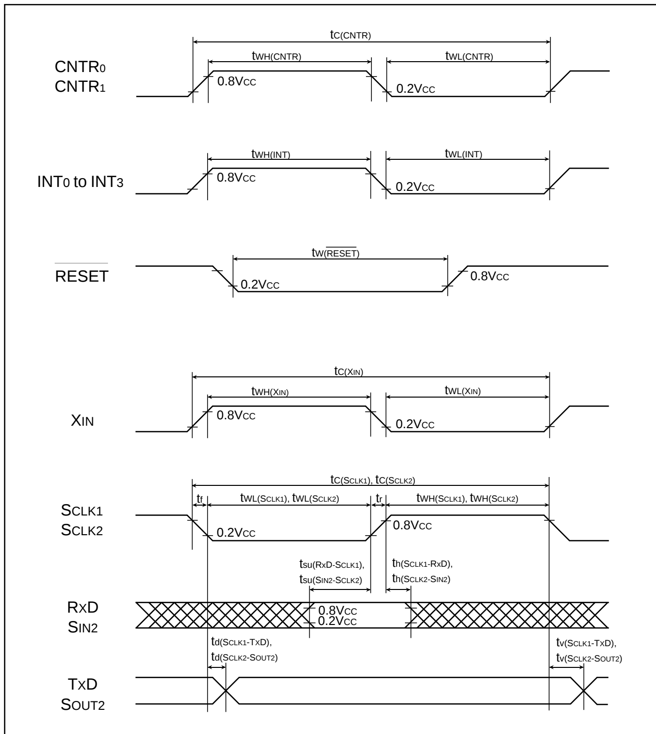
Fig. 84 Timing diagram
