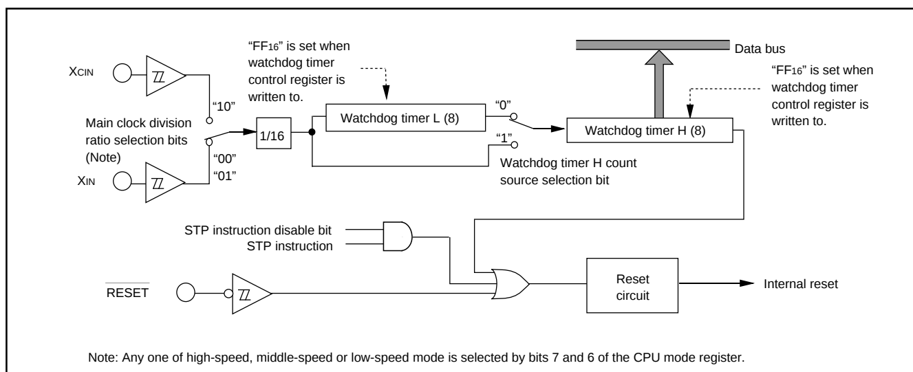
Fig. 54 Block diagram of Watchdog timer
