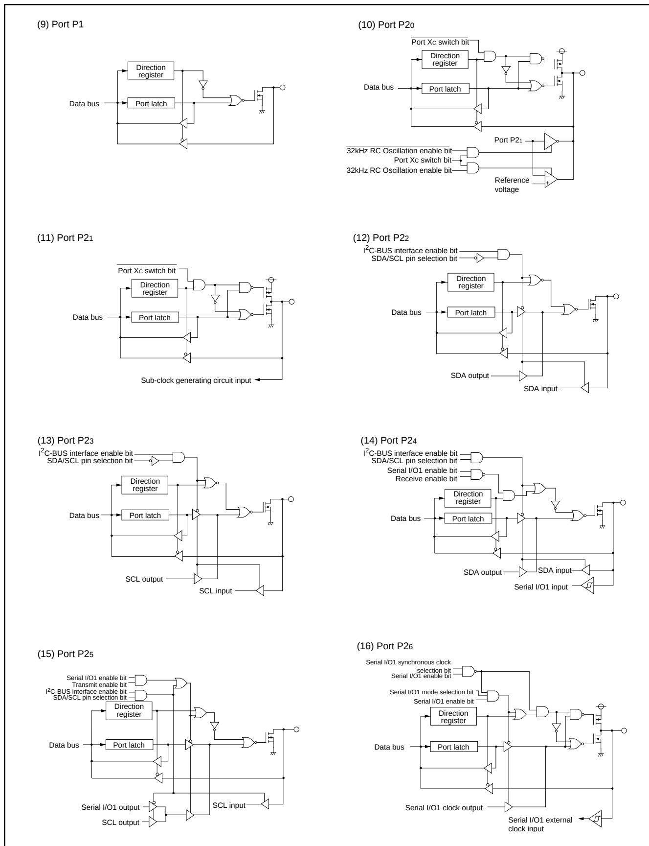
Fig. 10 Port block diagram (2)
