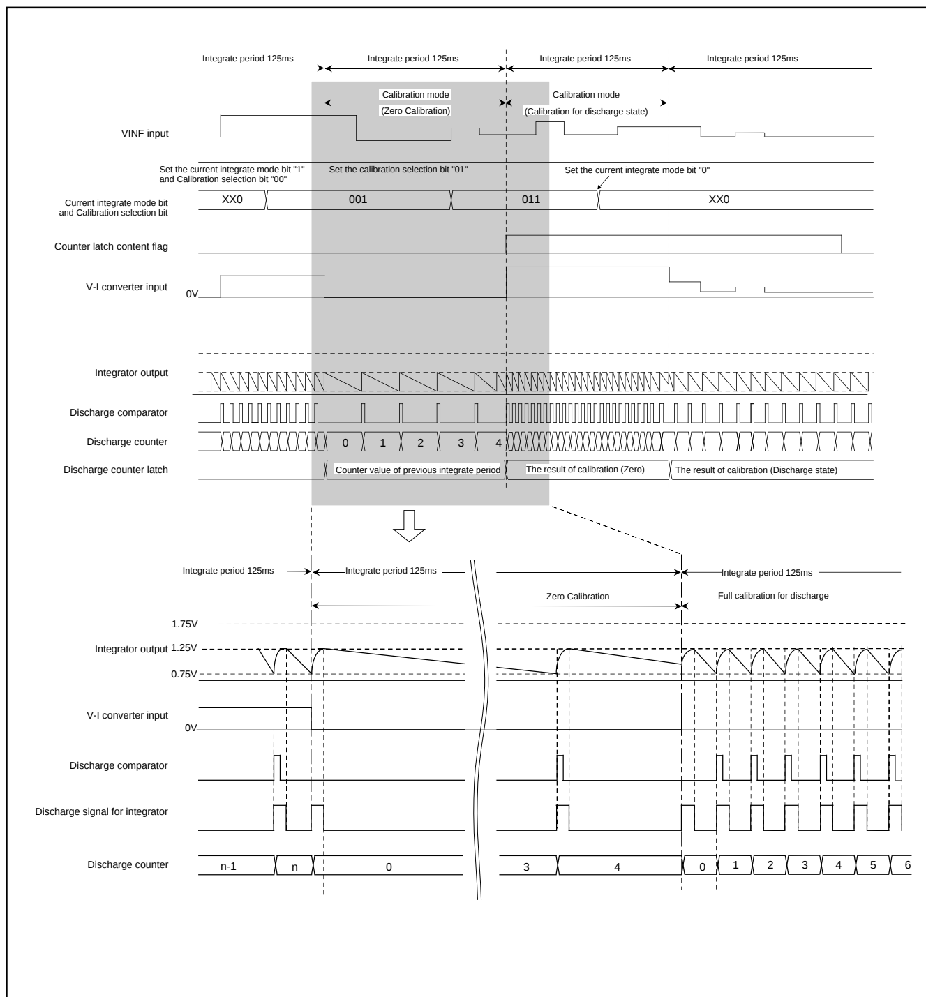
Fig. 49 Calibration timing
