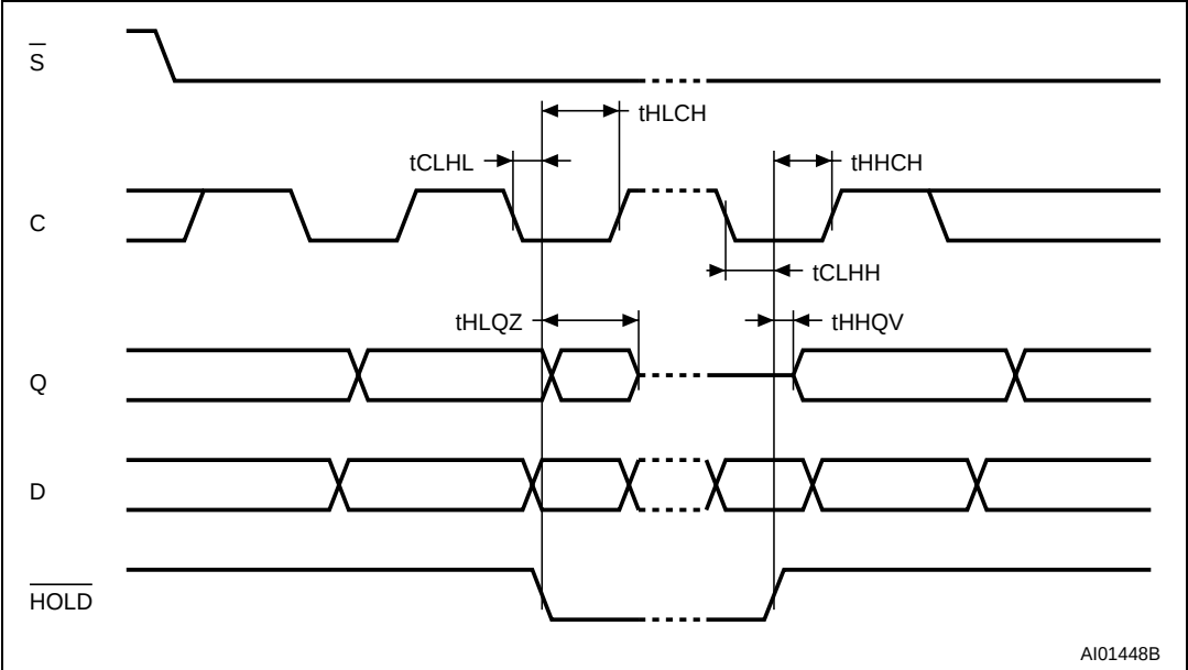
Figure 16. Hold timing
