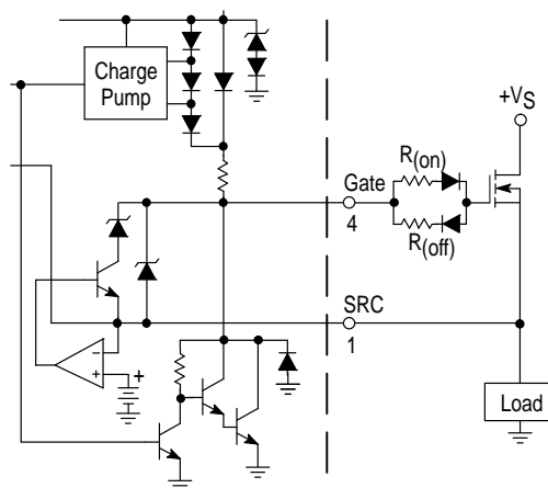
Figure 34. Independent Slow Down Adjustment of FET Turn-On and Turn-Off
