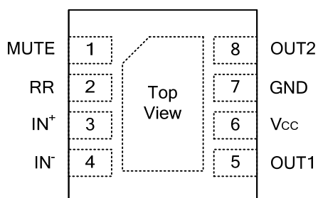
DFN3030-8
