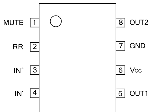
DIP-8/SOP-8 / TSSOP-8
