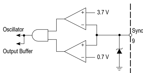
Figure 36. Synchronization
