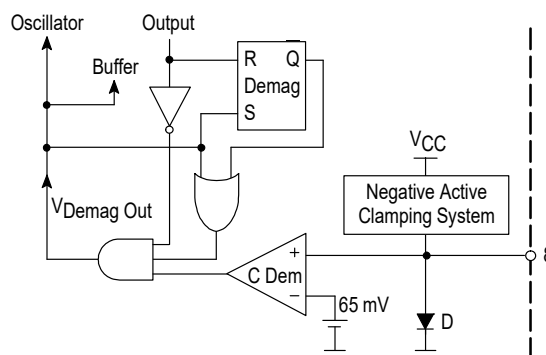
Figure 38. Demagnetization Block
