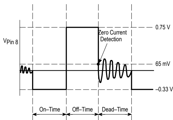
Figure 37. Demagnetization Detection
