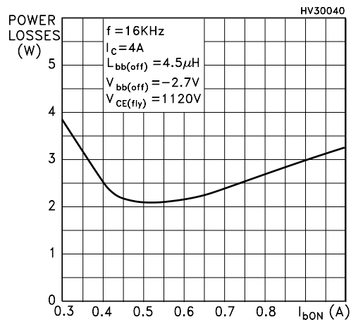
Figure 9. Power losses
