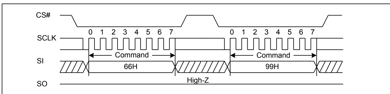
Figure 39. Enable Reset and Reset command Sequence Diagram
