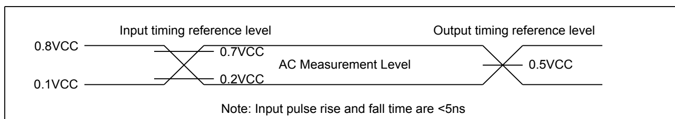
Figure 43. Input Test Waveform and Measurement Level Diagram
