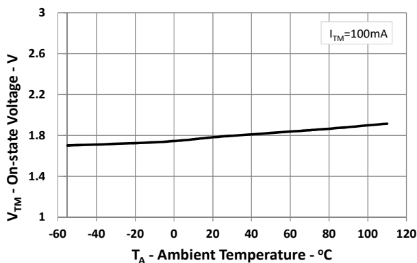
Fig.5 On-state Voltage vs. Ambient Temperature
