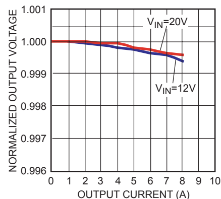
Load Regulation
