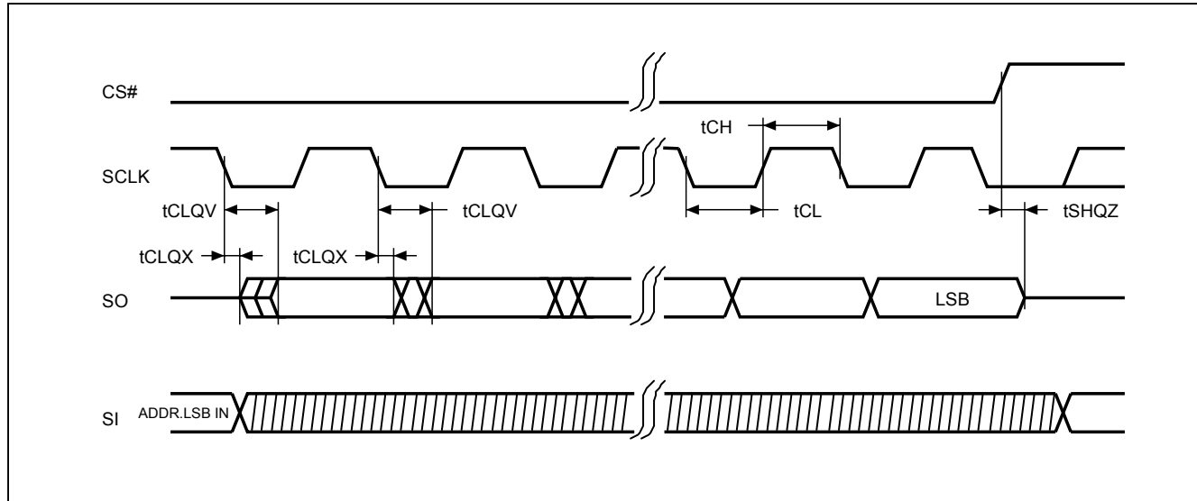
Figure 44. Output Timing
