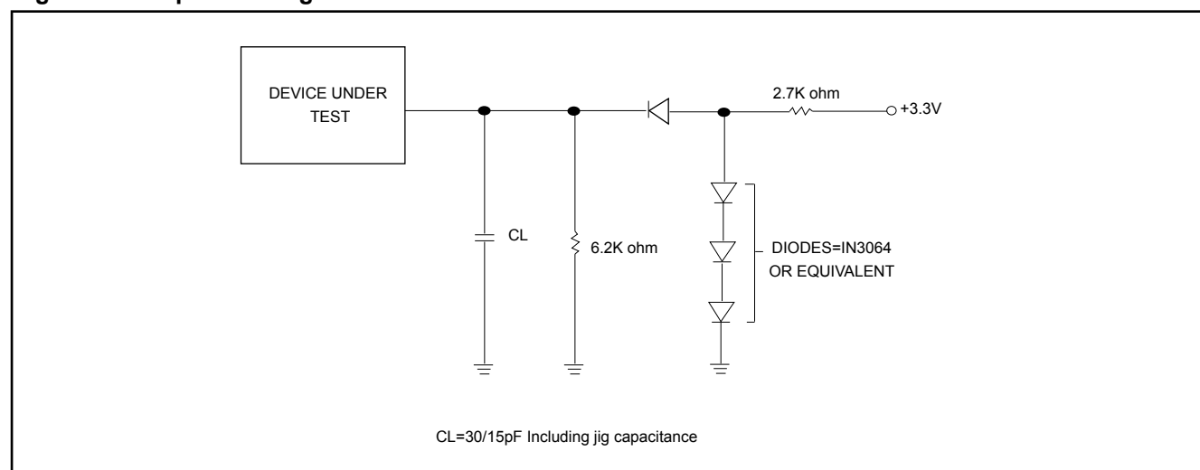
Figure 41. Output Loading
