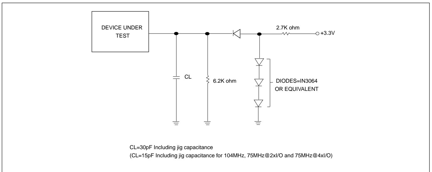
Figure 5. OUTPUT LOADING
