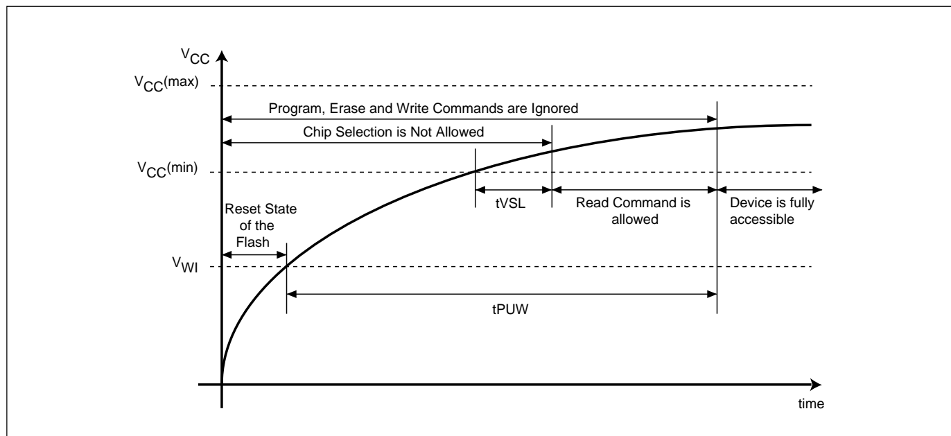
Figure 29. Power-up Timing
