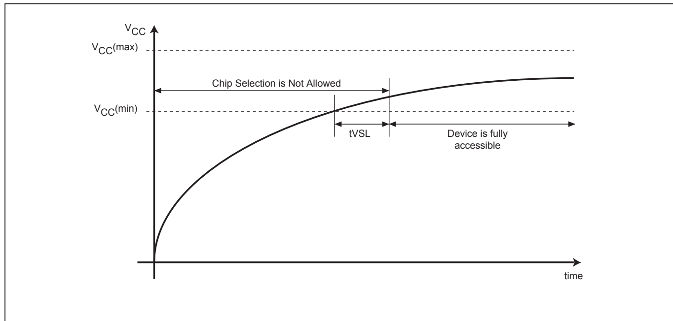
Figure 26. Power-up Timing
