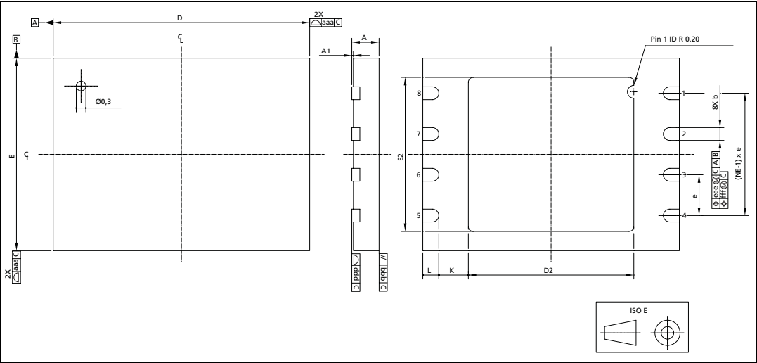
Figure 111. VDFPN8 (MLP8) Very Thin Dual Flat Package No Leads, 8×6x1 mm Drawing
