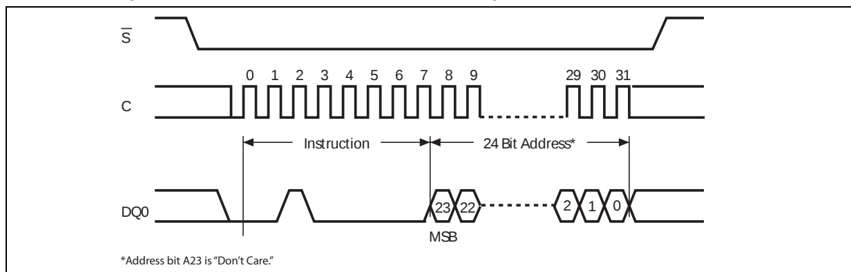
Figure 28. Subsector Erase instruction sequence
