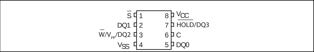
Figure 2. SO8N, SO8W and MLP8 connections
