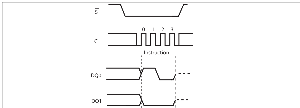
Figure 63. Clear Flag Status Register instruction sequence DIO-SPI
