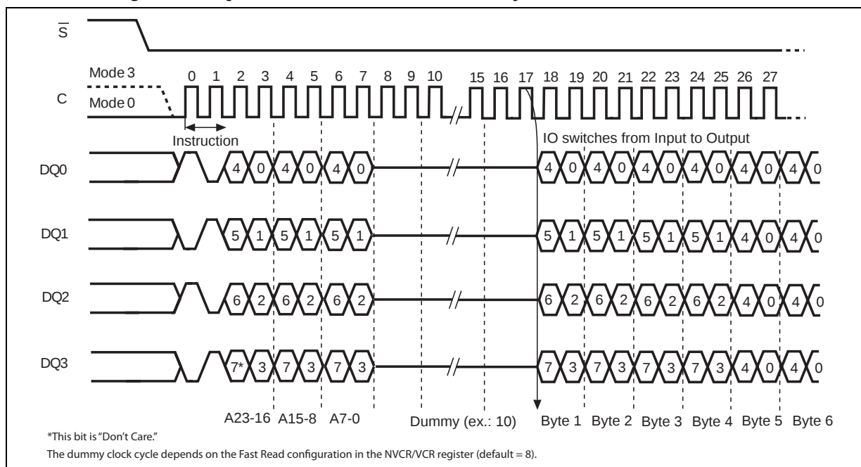
Figure 71. Quad Read Serial Flash Discovery Parameter
