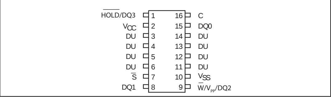
Figure 3. SO16 connections
