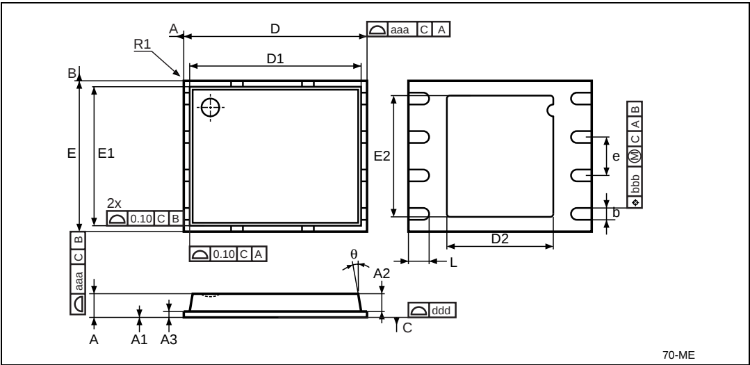
Figure 110. VDFPN8 (MLP8) Very Thin Pitch Dual Flat Package, No Leads, 6×5 mm Drawing
