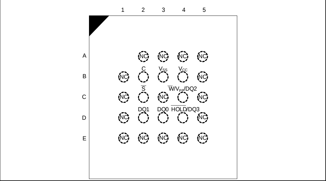
Figure 4. BGA connections
