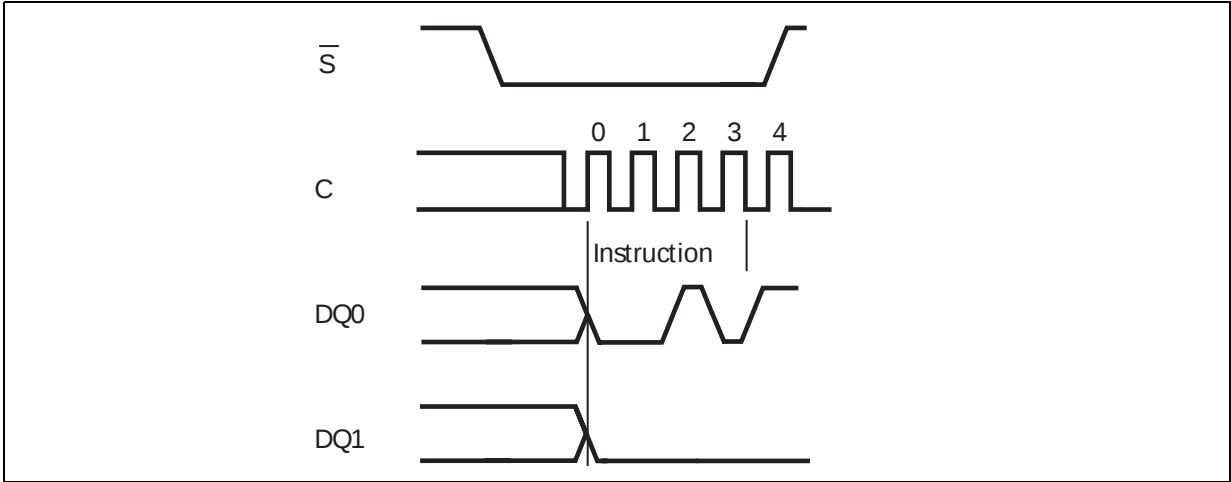
Figure 48. Write Disable instruction sequence DIO-SPI
