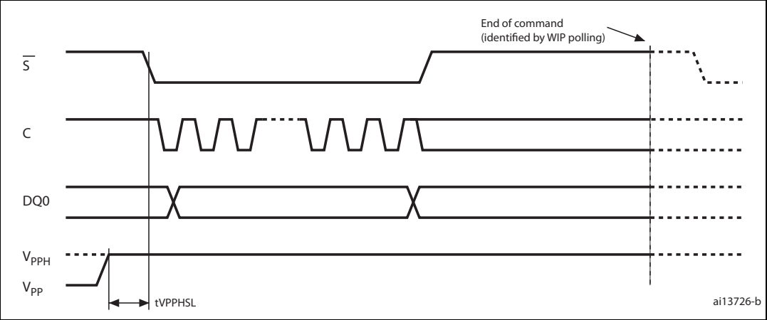
Figure 109. V_{PPH} timing
