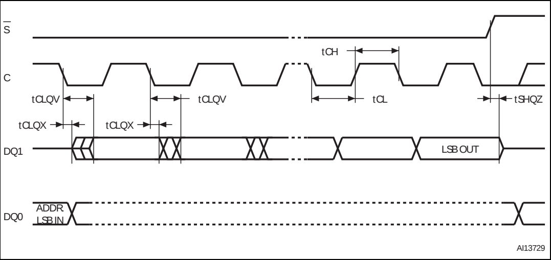
Figure 108. Output timing
