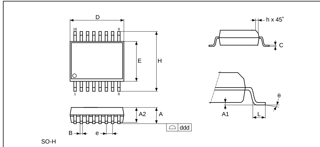
Figure 113. SO16 Wide – 16 Lead Plastic Small Outline, 300 mils Body Width, Drawing
