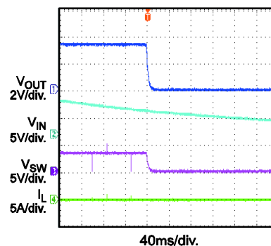
Shut-Down through VIN
