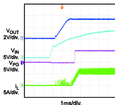
Power Good through VIN Start-Up
