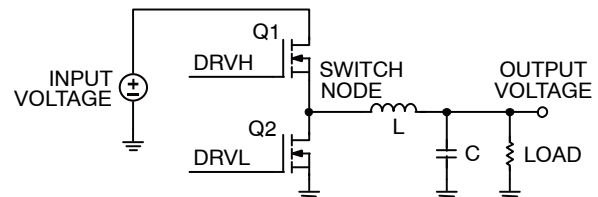
Figure 22. Buck Topology
