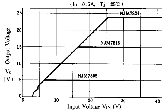
NJM7805 Dropout Characteristics
