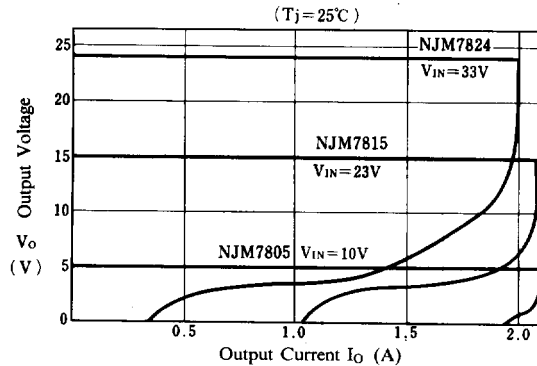
NJM7805/15/24 Load Characteristics
