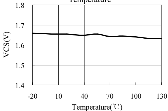
Current Sense Threshold Clamping vs Temperature
