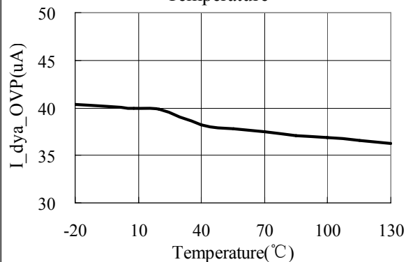
Dynamic OVP Triggering Current vs Temperature
