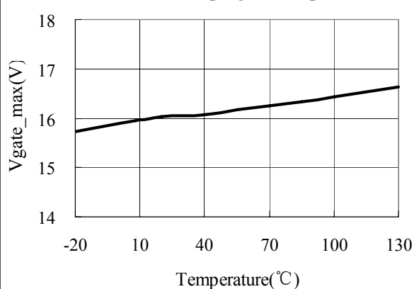
Gate Driver Clamping vs Temperature
