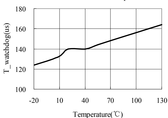
Restart Timer Period vs Temperature
