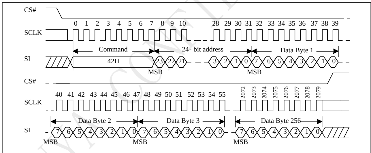
Figure 10-28 Program Security Registers (PRSCUR) Sequence (Command 42)
