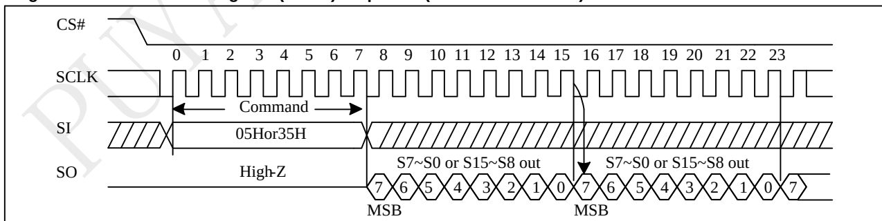
Status Register
