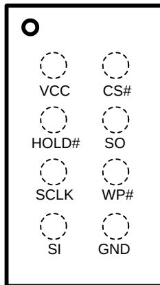
8-Ball WLCSP Ball Assignment
