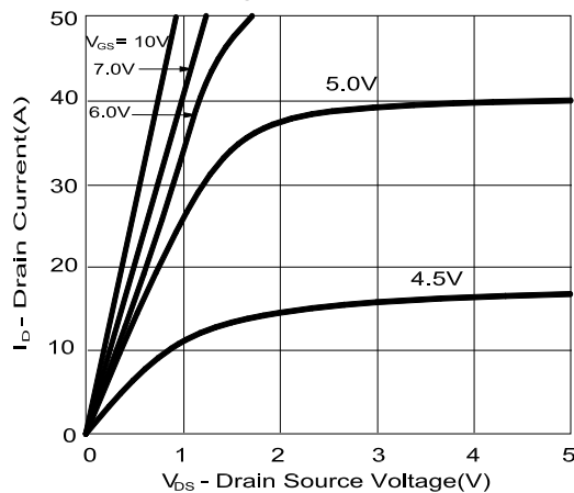
On-Region Characteristics
