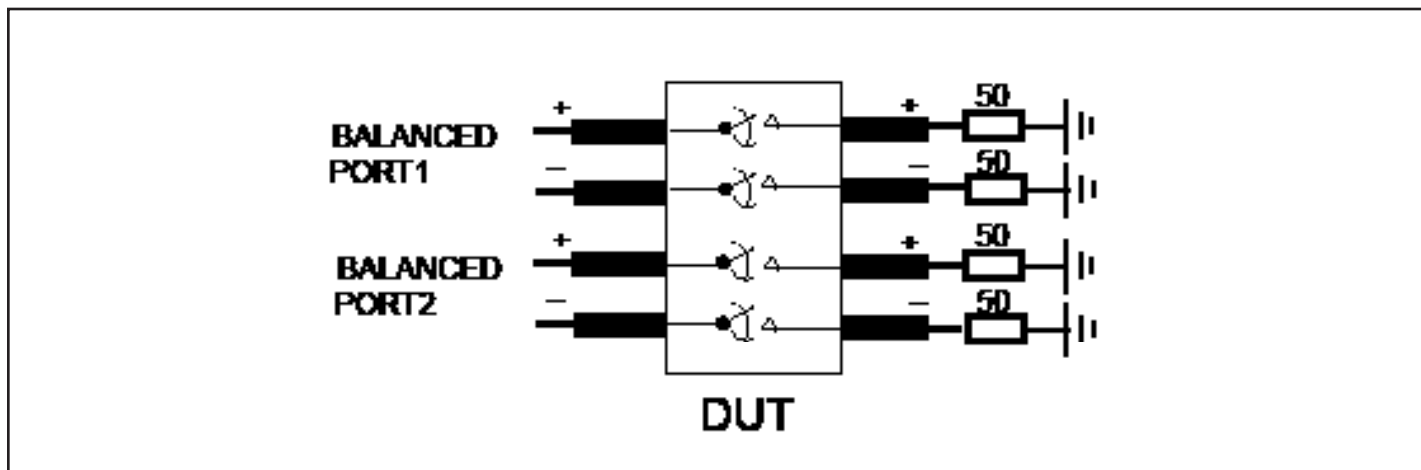
Fig 1. Crosstalk Setup
