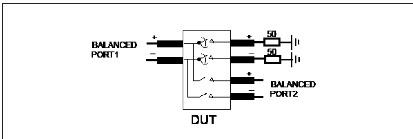
Fig 2. Off-isolation setup
