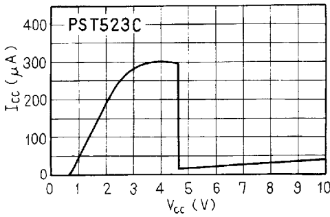
■ Vcc vs. Icc
