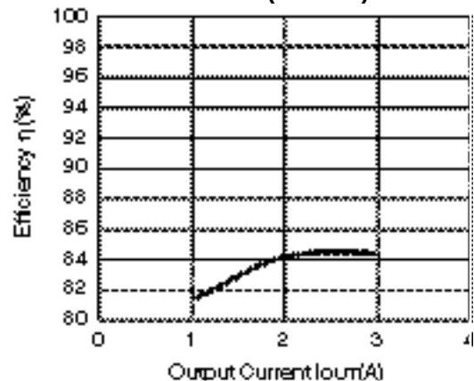
R1224N332M ( V_{IN}=18V )
