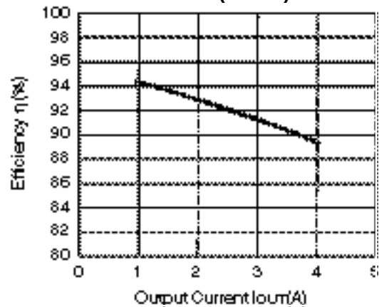
R1224N332M ( V_{IN}=5V )
