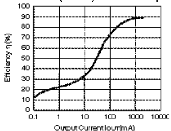
R1224N332M ( V_{IN}=12V ) CDRH127-27 \mu H
