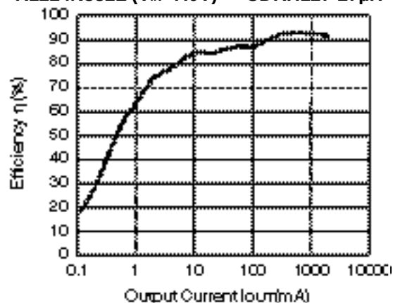
R1224N332L ( V_{IN}=7.0V ) CDRH127-27 \mu H
