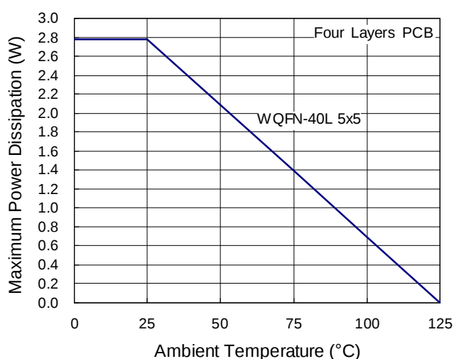
Figure 1. Derating Curves for RT9919 Packages
