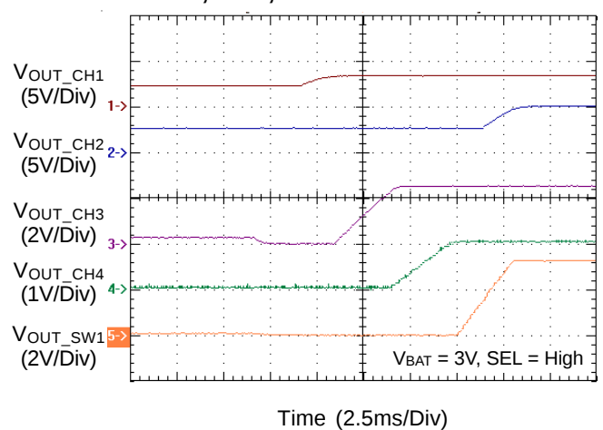
CH1, CH2, CH3 and CH4 Power On
