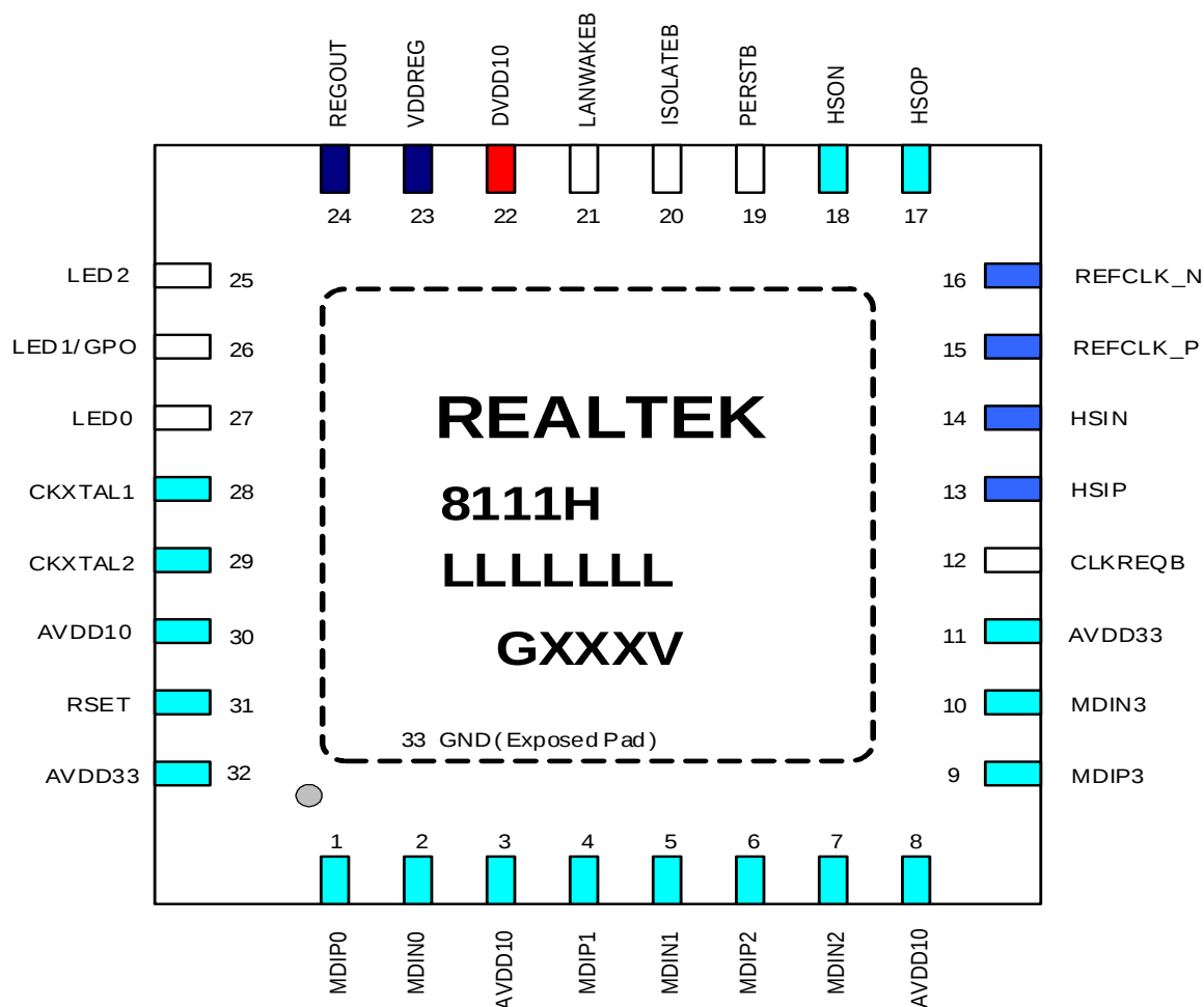
Figure 2. RTL8111H Pin Assignments
