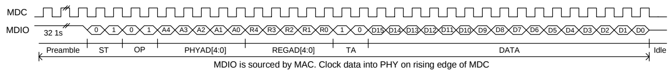
Figure 5. Write Cycle
