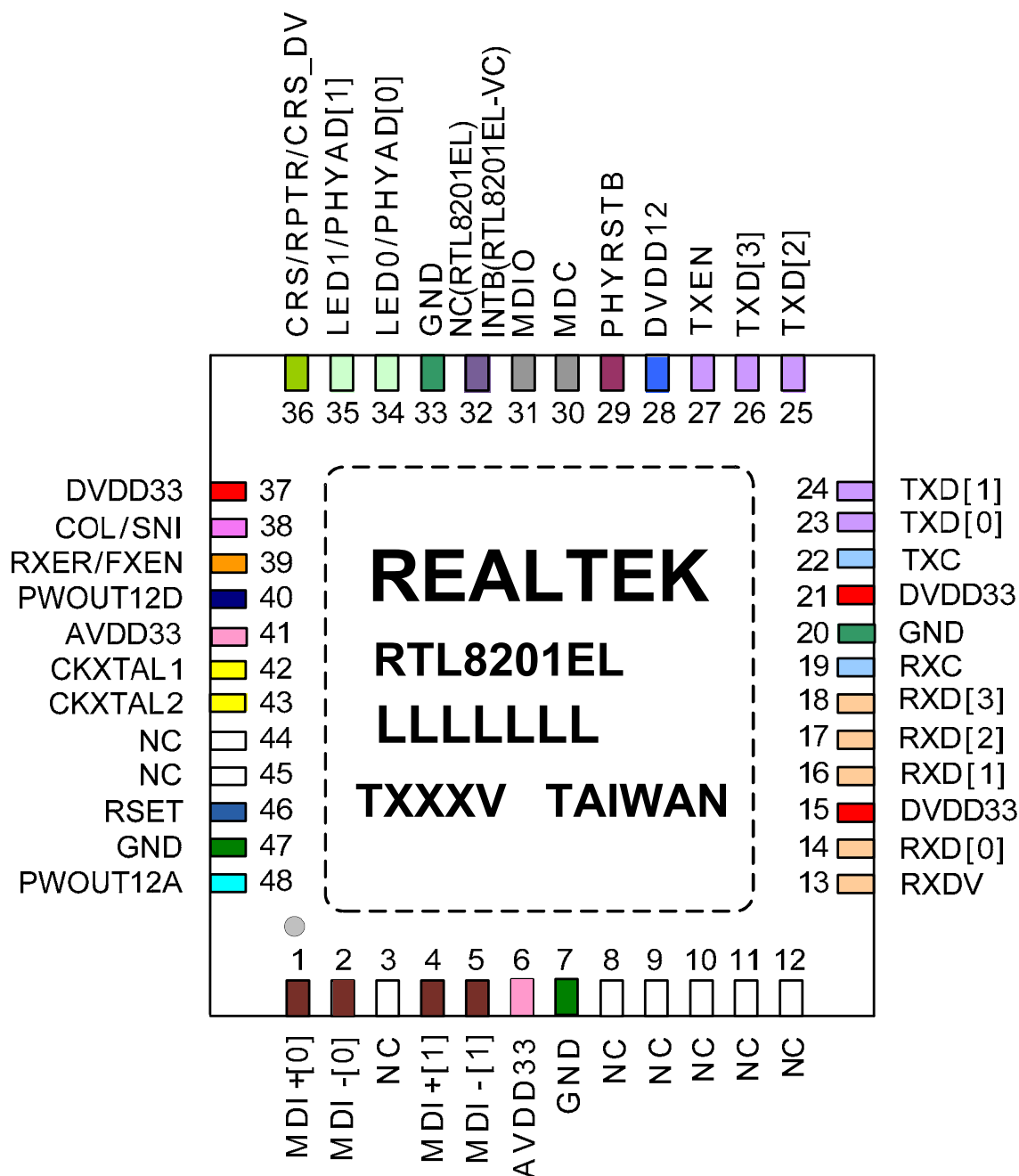
Figure 3. RTL8201EL LQFP-48 Pin Assignments
