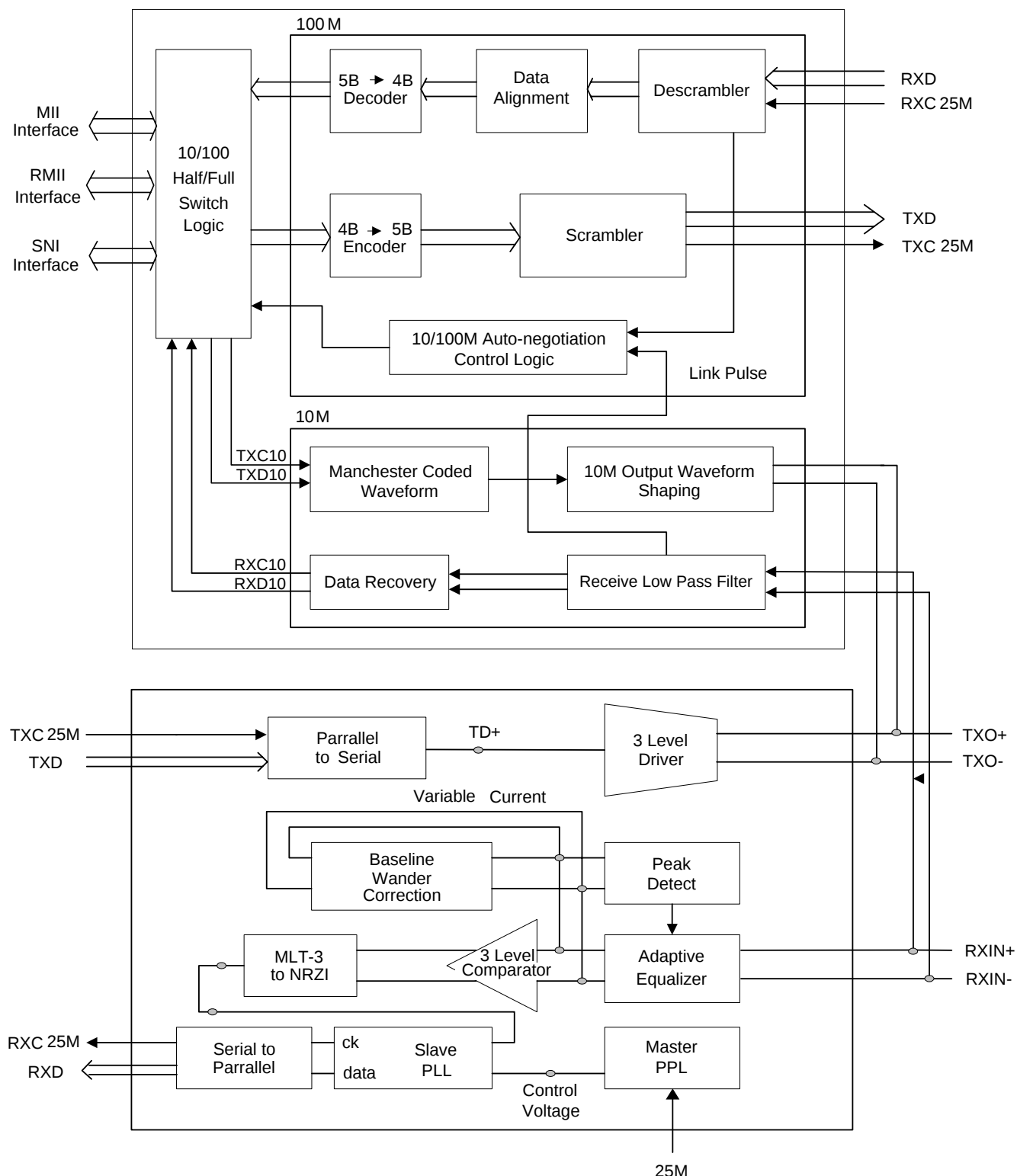
Figure 1. Block Diagram
