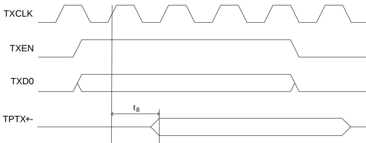
Figure 19. SNI Transmission Cycle Timing-2
