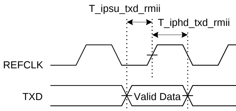
Figure 13. RMII Transmission Cycle Timing
