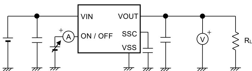
Figure 15 Test Circuit 4
