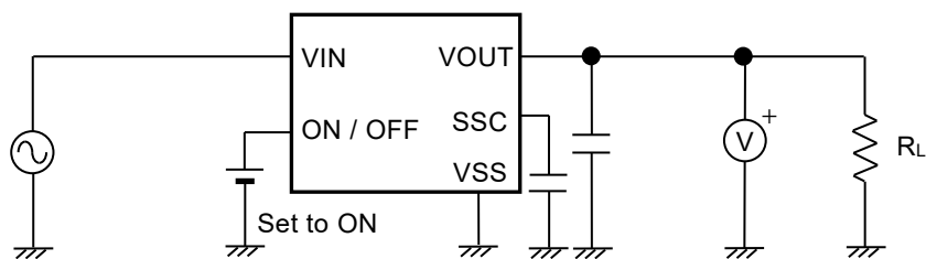
Figure 16 Test Circuit 5
