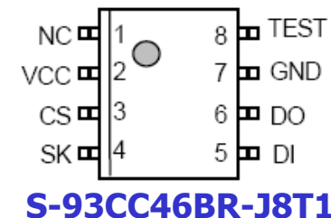
8-Pin SOP (JEDEC) (Rotated) Top view
