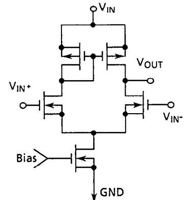
Figure 5 Error amplifier
