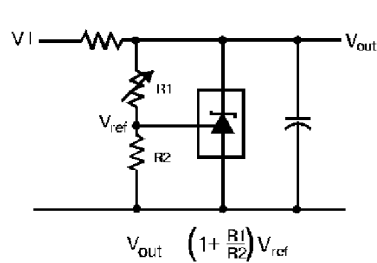
FIGURE 1. SHUNT REGULATOR
