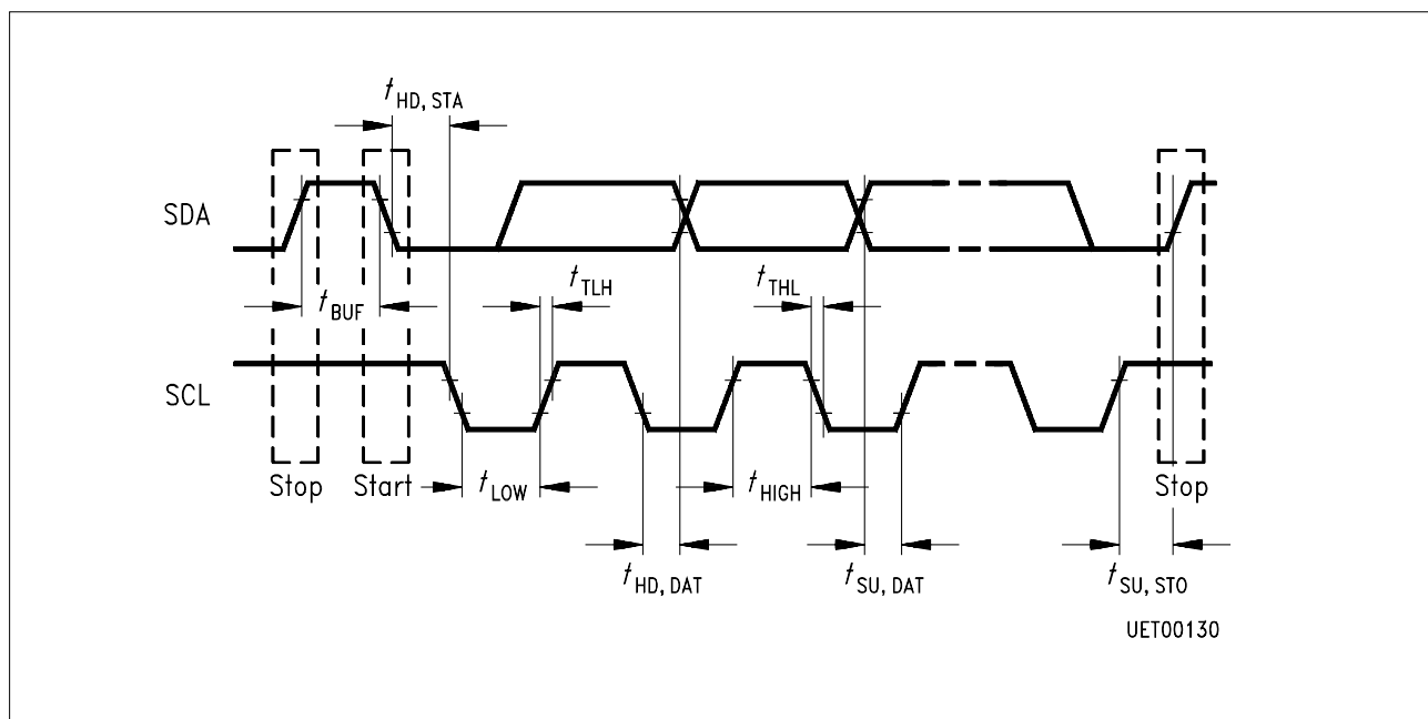
Figure 3 I²C-Bus Timing
