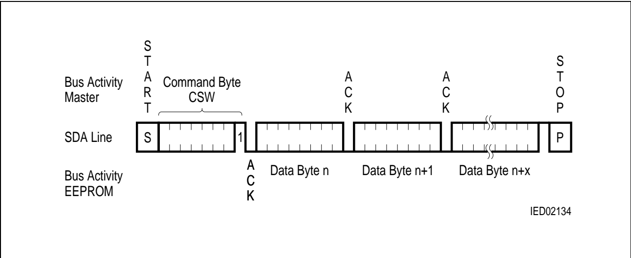
Figure 13 Sequential Read
