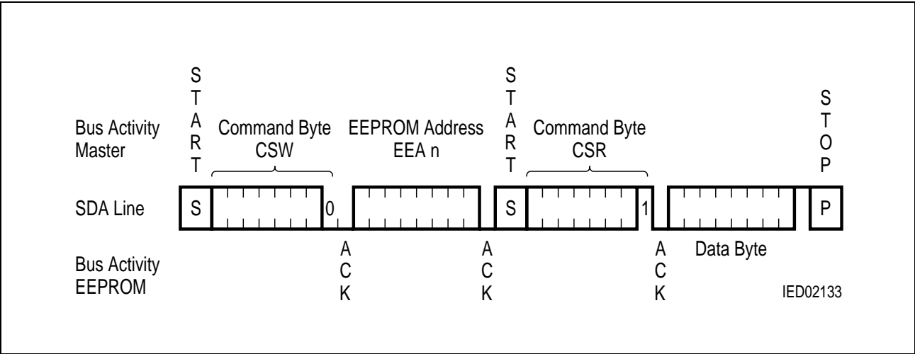
Figure 11 Random Read
