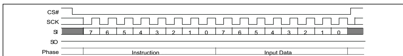
Figure 55 Bank register write (BRWR 17h) command
