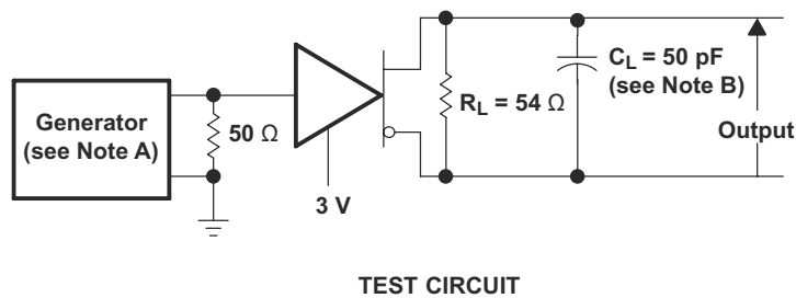
Figure 7-3. Driver Test Circuit and Voltage Waveforms
