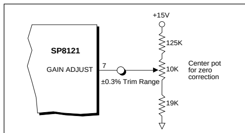
Figure 2. Gain Adjust
