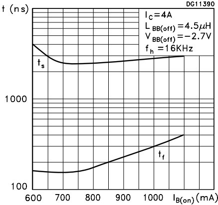
Figure 8. Switching time inductive load
