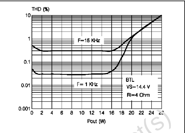
Figure 19. Distortion vs output power
