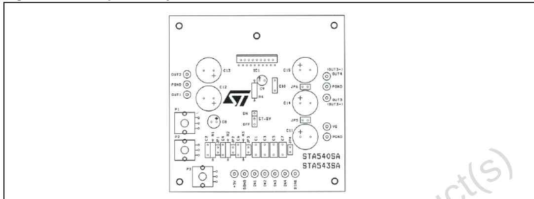
Figure 5. Component layout
