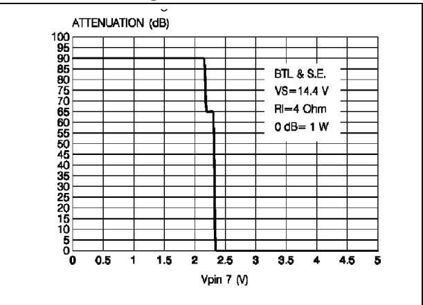
Figure 23. Standby attenuation vs threshold voltage
