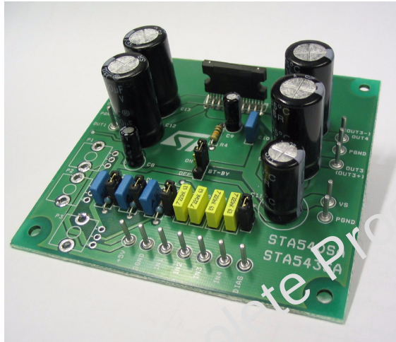
Figure 3. Test and application board
