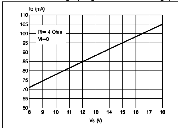
Figure 12. Quiescent drain current vs supply voltage (single-ended and bridge)
