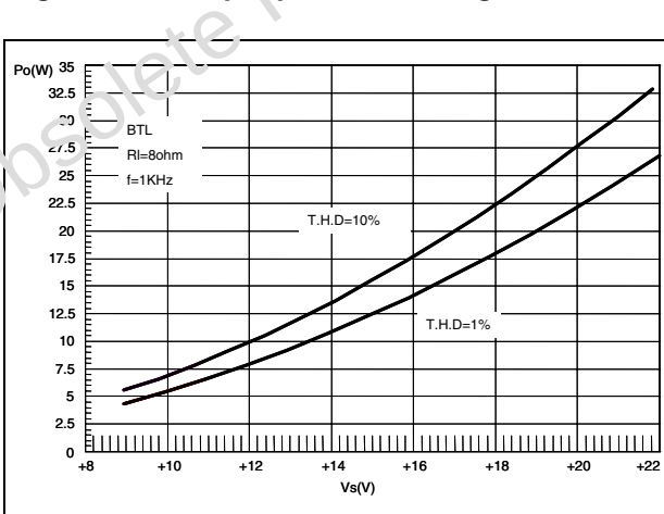
Figure 22. Output power vs voltage
