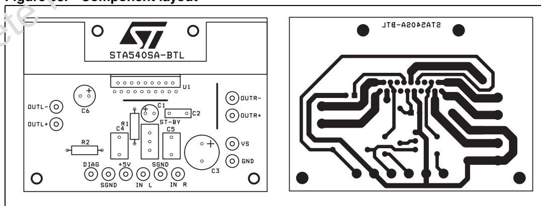
Figure 38. Component layout
