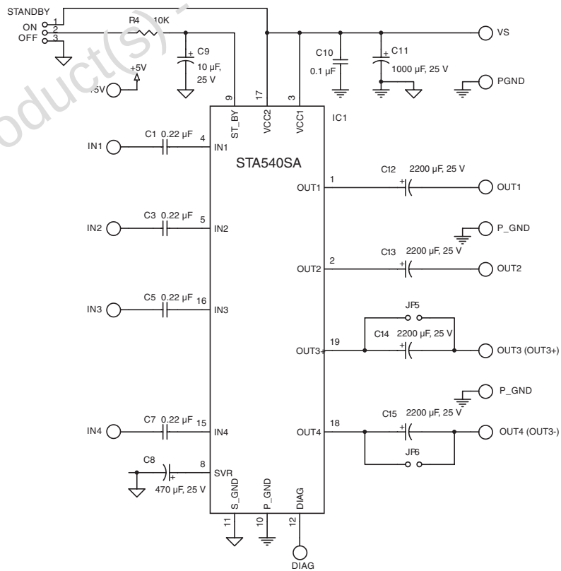
Figure 4. Test circuit
