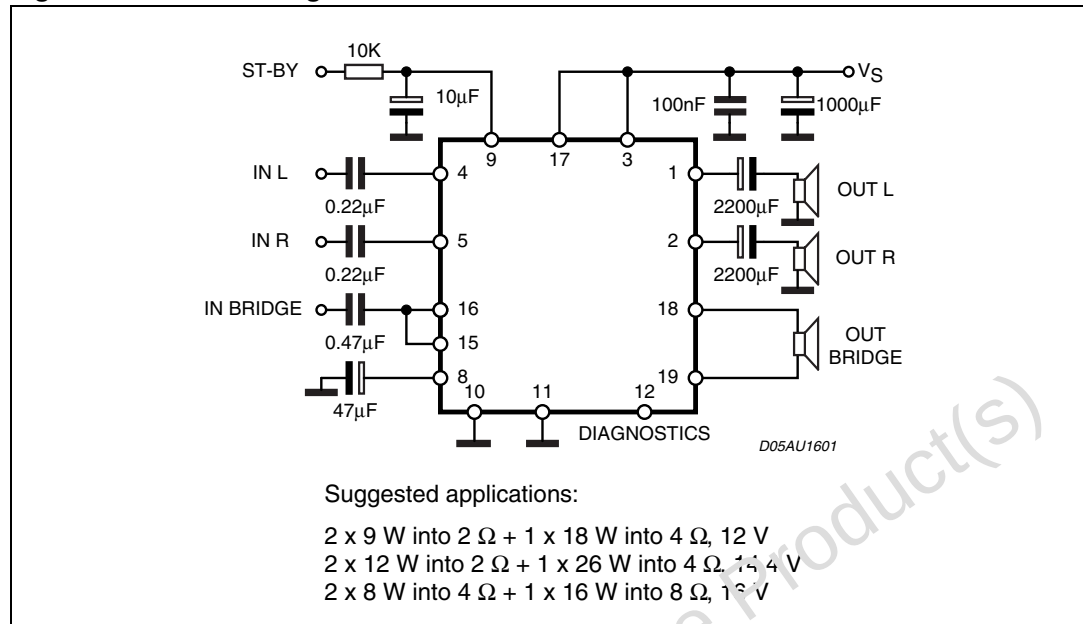
Figure 11. Stereo Bridge
