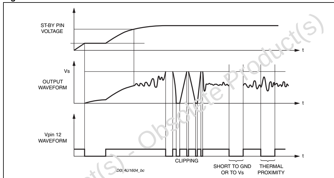
Figure 33. Waveforms
