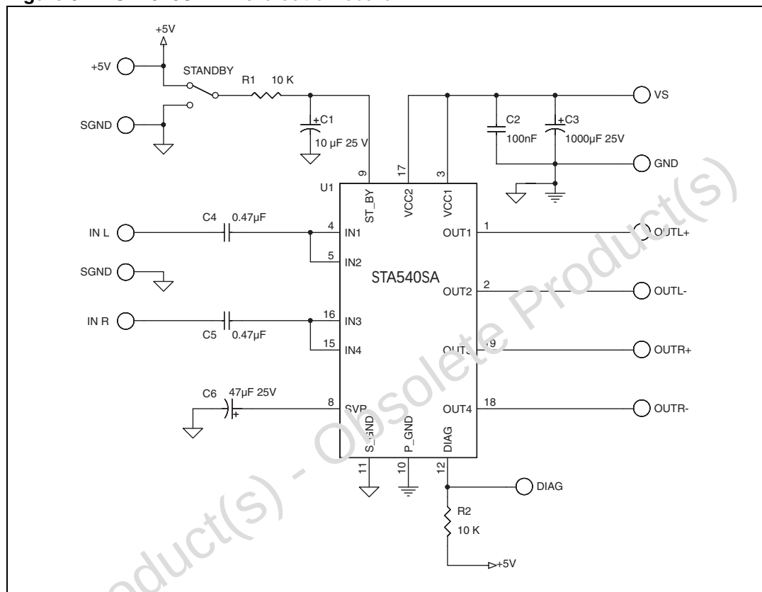
Figure 37. STA540SA-BT evaluation board
