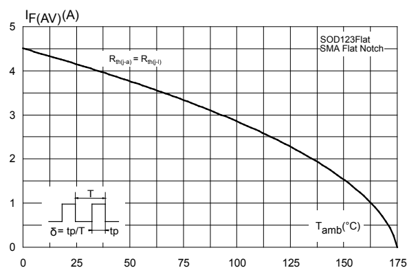
Figure 4. Average forward current versus ambient temperature (SOD123Flat, SMA Flat Notch, \delta = 0.5 )
