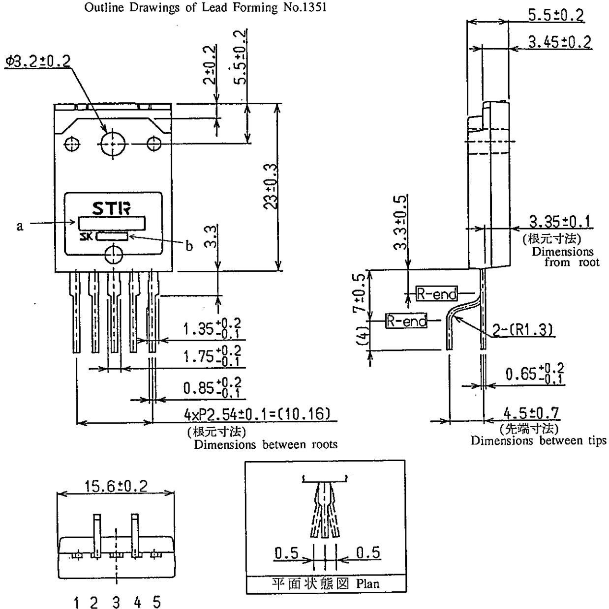
STR-F 外形寸法図 LF1351 Outline Drawings of Lead Forming No.1351
