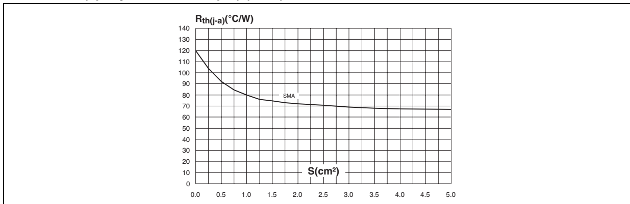
Figure 15. Thermal resistance junction to ambient versus copper surface under each lead (epoxy FR4, \text{Cu} = 35 \mu\text{m} ) (SMA)
