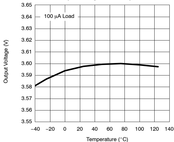
Output Voltage 2 vs. Temperature
