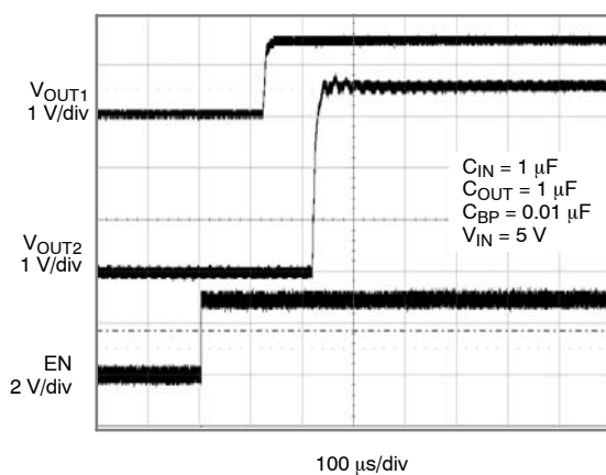
Enable Sequence
