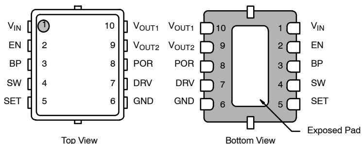
PowerPAK MLP33-10
