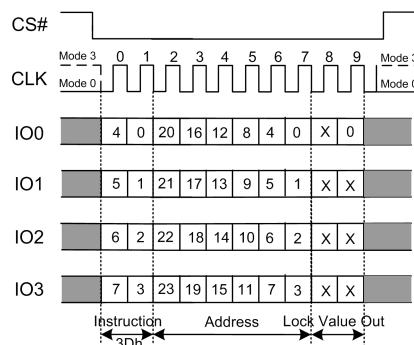
Figure 7.38b Read Block Lock Instruction(QPI Mode)
