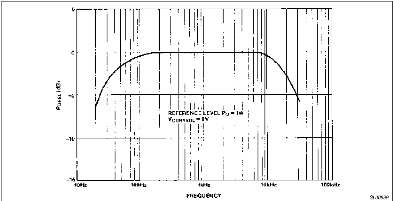
Figure 12. Frequency Characteristic
