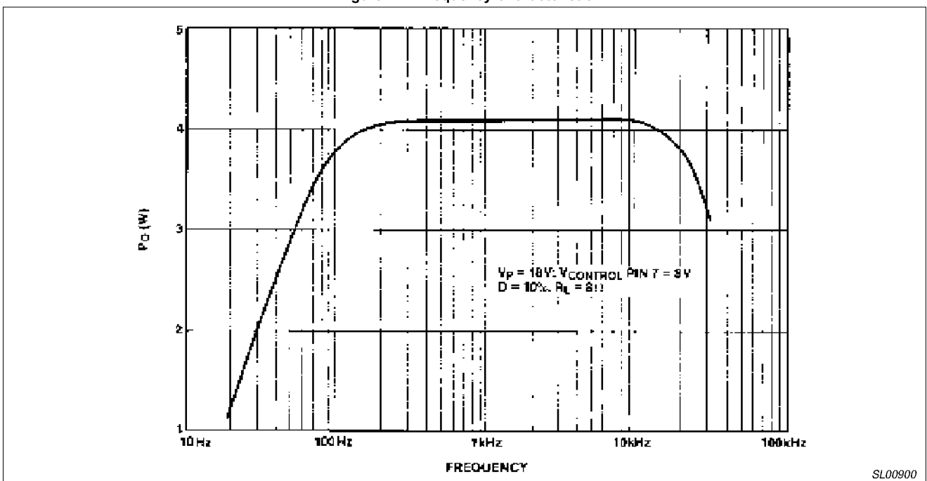
Figure 13. Power Bandwidth
